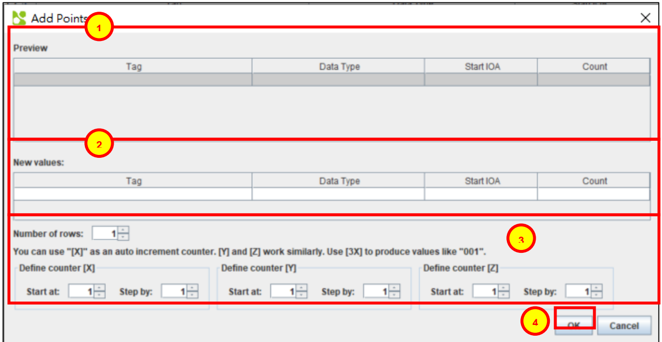
Figure 3-4 – Adding Data Points to an IEC 60870-5-101 Remote IED.
