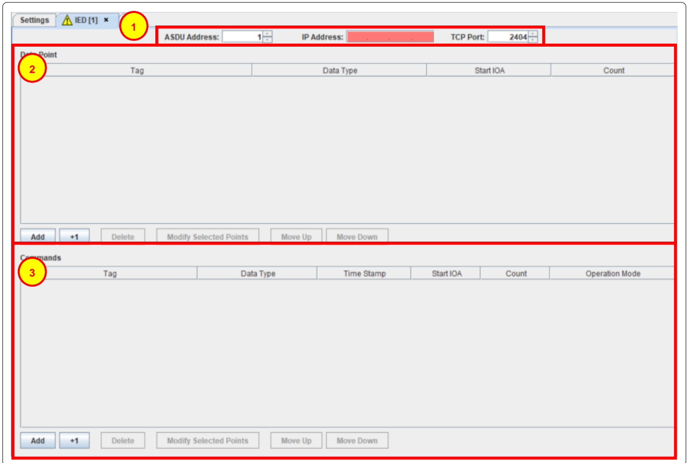
Figure 4-3 – IED configuration settings for an IEC 60870-5-104 Client.
