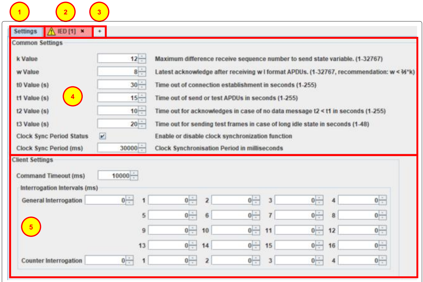
Figure 4-1 – Configuration Settings for the IEC 60870-5-104 Client.
