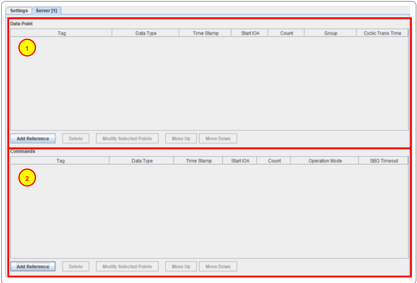
Figure 4-9 – IED configuration settings for an IEC 60870-5-104 Server.
