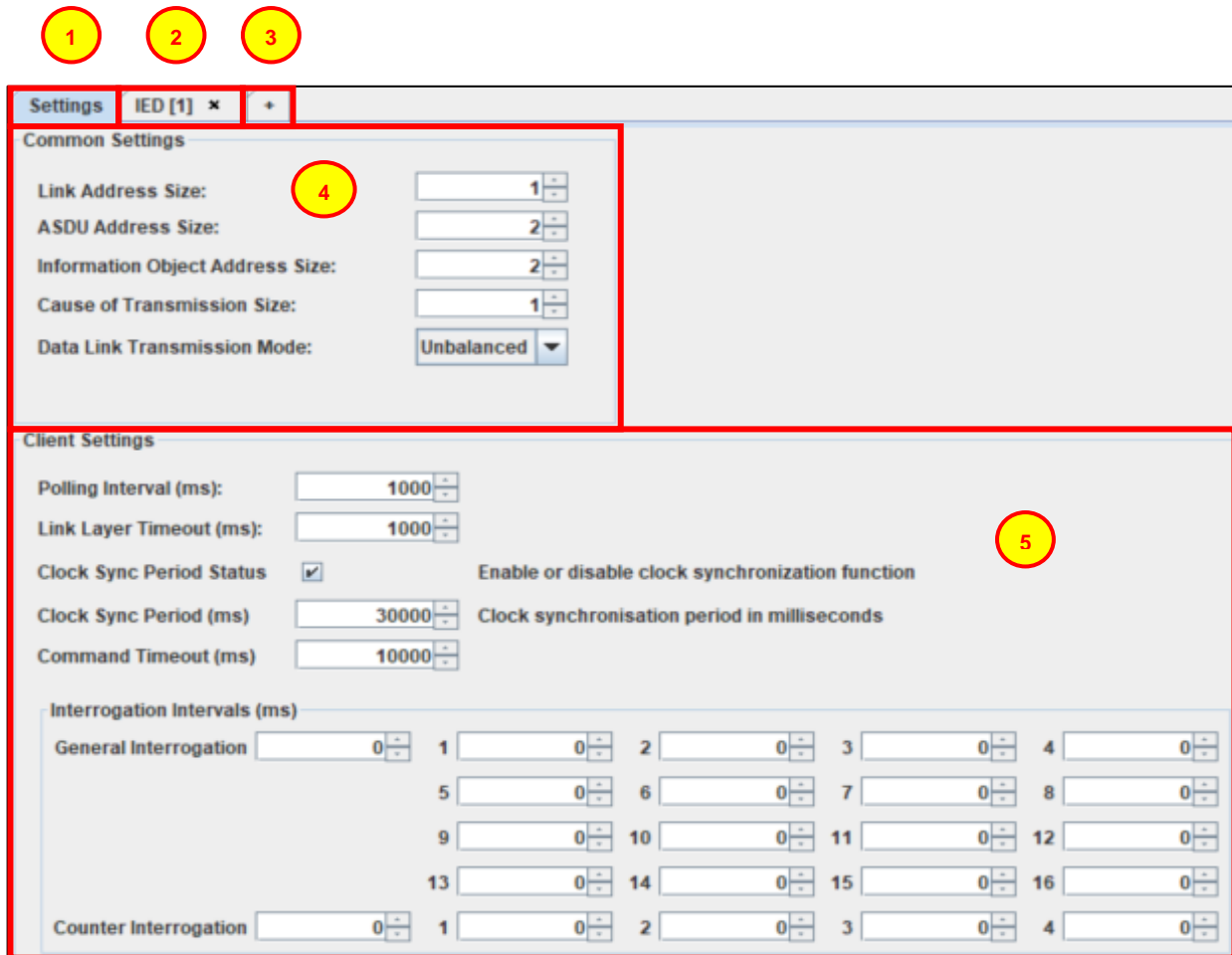
Figure 3-1 – Configuration Settings for the IEC 60870-5-101 Client.
