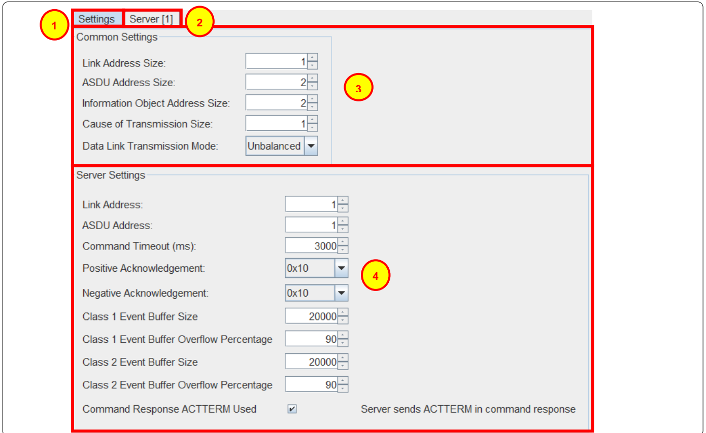
Figure 3-7 – Configuration settings for a local IEC 60870-5-101 Server.
