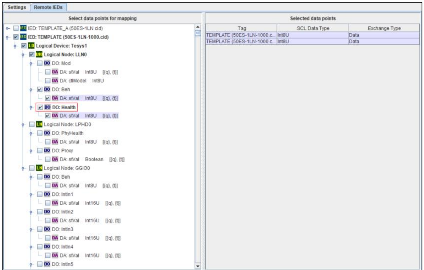
Figure 2-2 - Main screen.
