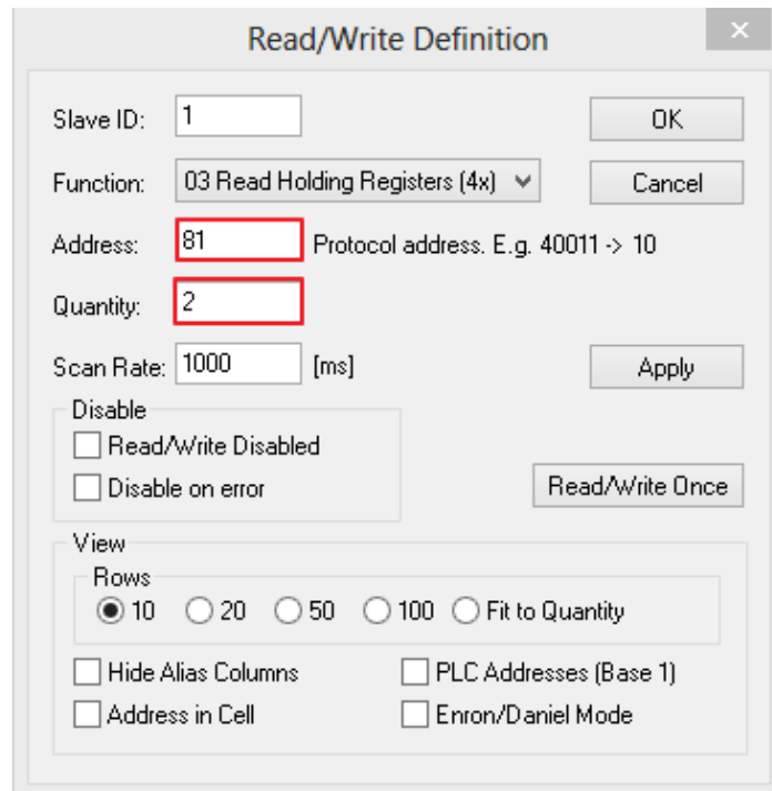
Figure 2.127 Setup Starting Address and Quantity in Modbus Poll
