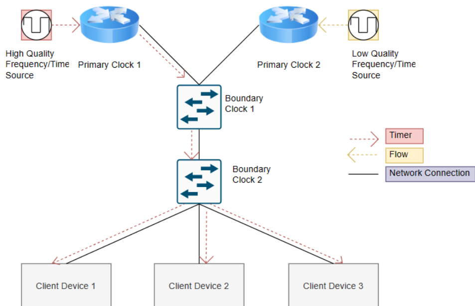
Figure 2.121 Network Diagram of Precision Time Protocol (PTP)
