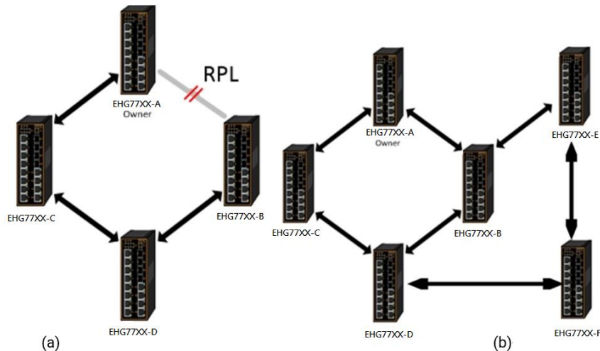
Figure 2.21 An Example of Ring Topology (a) Major Ring, and (b) Sub-Ring
