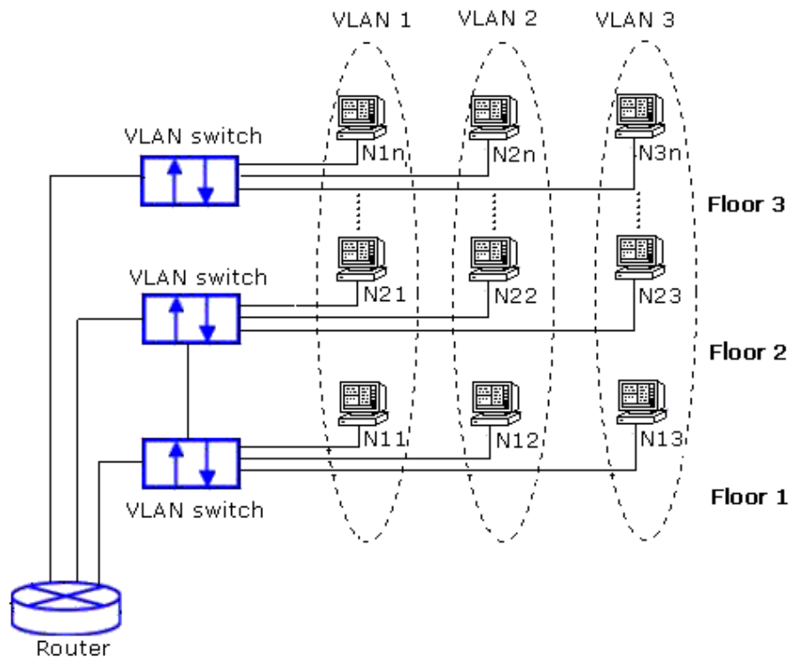
Figure 2.95 Example of VLAN Configuration
