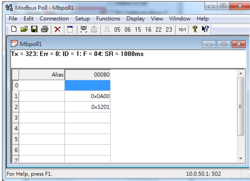
Figure 2.128 Modbus Memory Address 81 and 82 are the location of EHG77XX's IP Address
