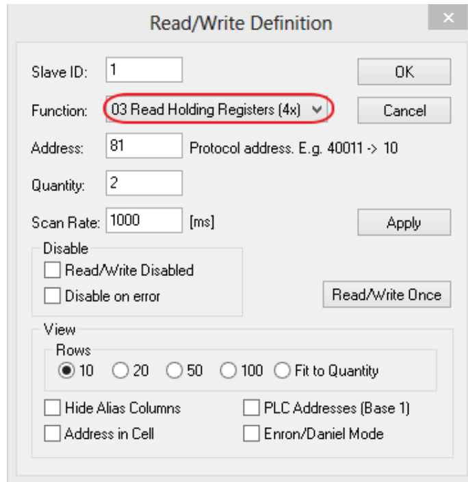
Figure 2.126 Set Code 03 in the Modbus Poll Function
