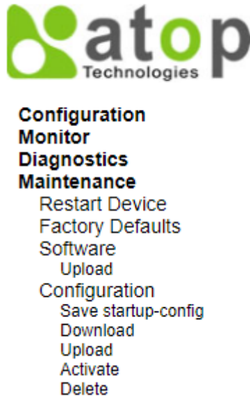
Figure 5.1 Maintenance Menu
