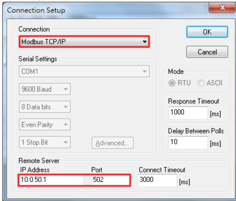
Figure 2.121 Modbus Poll Connection Setup
