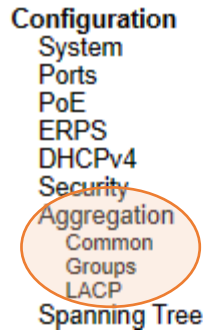
Figure 2.77 Configuration->Aggregation Submenus
